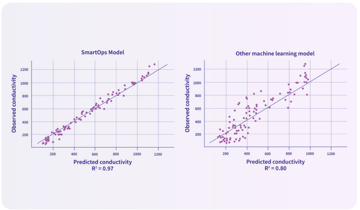
Figure 5: Prediction using (a) SmartOps model and (b) other ML model
