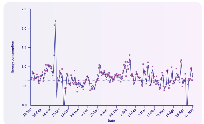
Figure 6: Energy Consumption of the Treatment Plant
