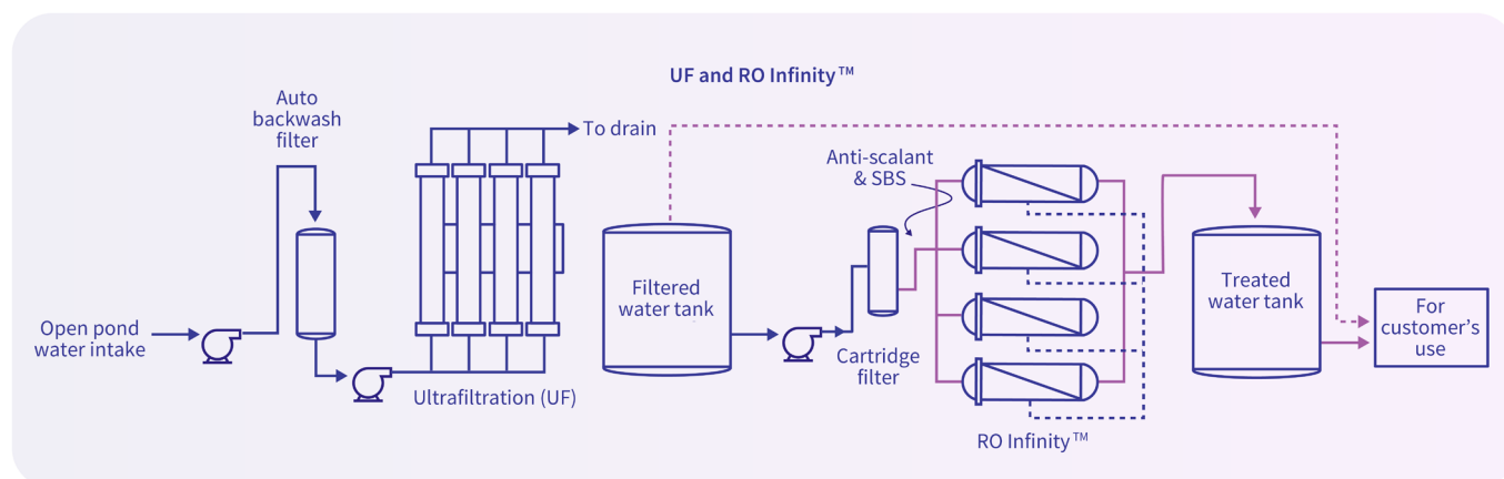
Figure 1: Process Flow Diagram for the Treatment Plant
