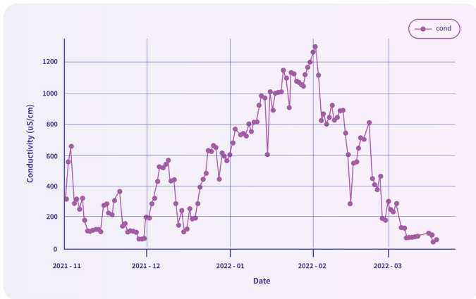
Figure 4: Conductivity of Open Pond Water Intake
